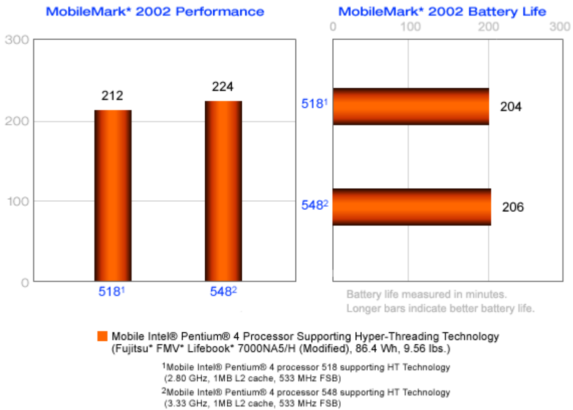
Figure 1. Mobile Intel® Pentium® 4 Processor Supporting Hyper-Threading Technology Performance and Battery Life on MobileMark* 2002
